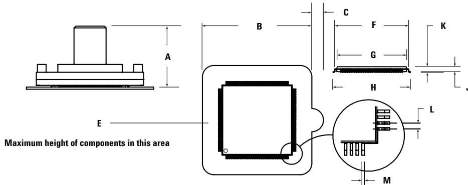
Figure 16. Elastomeric probe and package dimensions for TQFP
