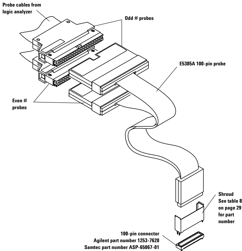
Figure 32. Agilent E5385A connection and pinout
