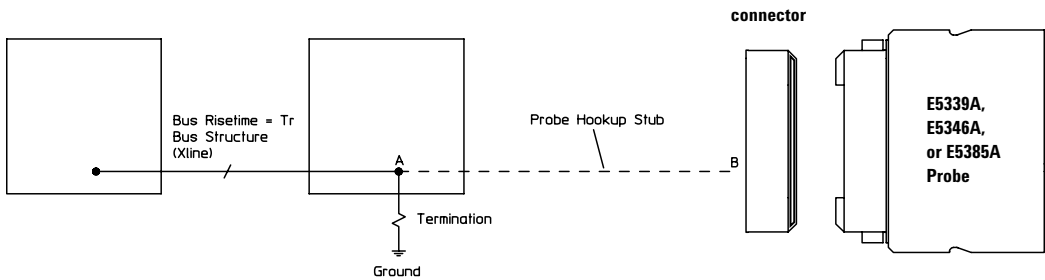
Figure 31. Agilent E5339A, E5346A, and E5385A design rules
