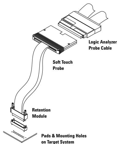
Figure 40. E5387A soft touch differential probe
