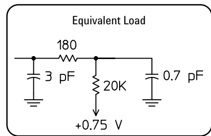
Figure 55. E5380A input equivalent load, including 38-pin connector
