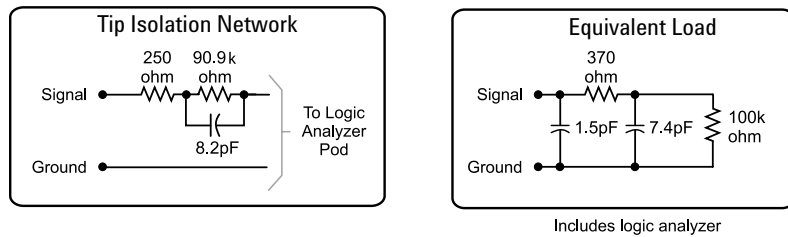
Figure 3. Probe tip isolation network and equivalent load
