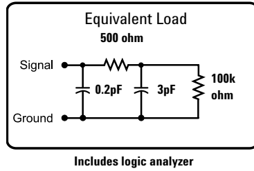
Figure 61. Equivalent load for high-speed general-purpose probe
