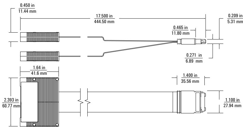
Figure 25. E5346A, E5351A, E5339A mechanical dimensions
