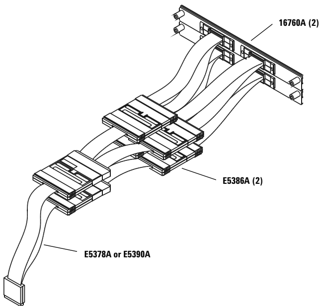
Figure 47. E5386A with E5378A or E5390A single-ended probe.
