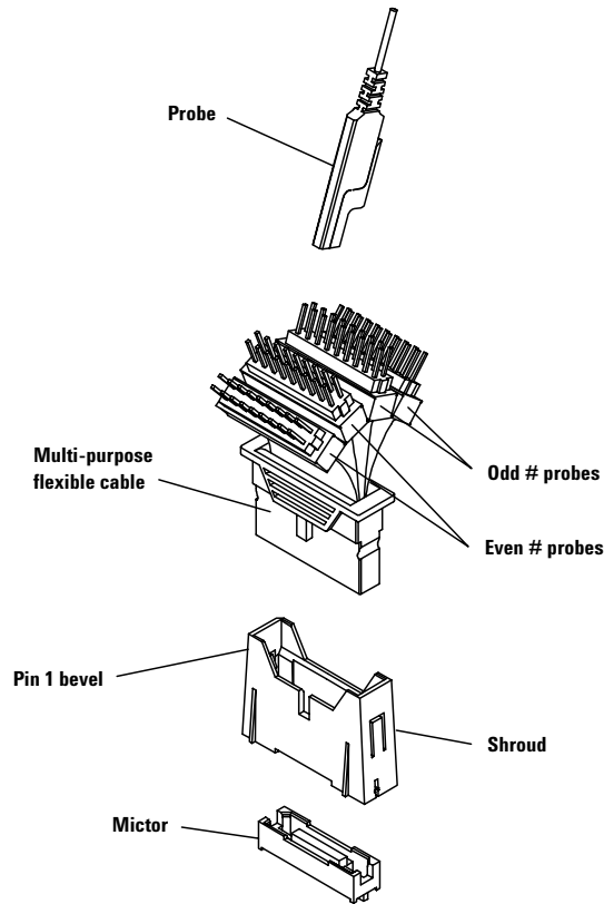
Figure 37. E5346-60002 Mictor break-out adapter
