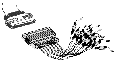
Figure 4. Sixteen-channel probe lead set (part number 01650-61608)
