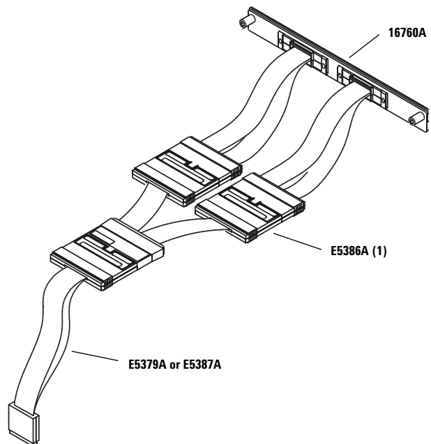
Figure 48. E5386A with E5379A or E5387A differential probe.
