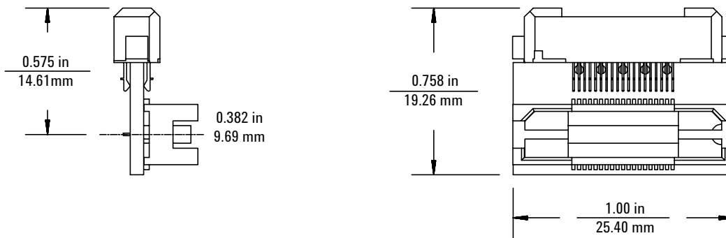
Figure 38. E5346-63201 right-angle 38-pin adapter
