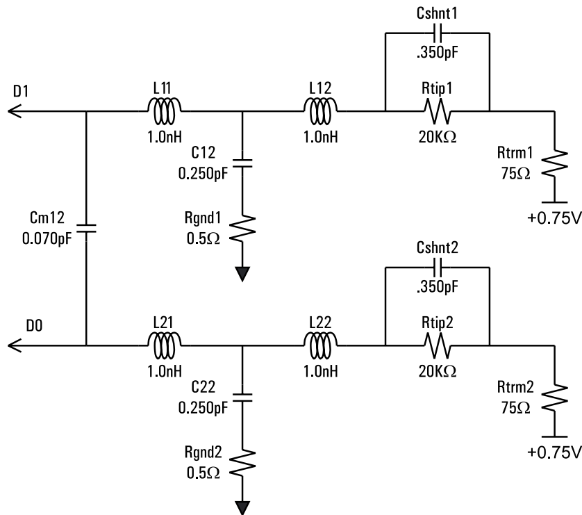
Figure 43. Load model for soft touch probes
