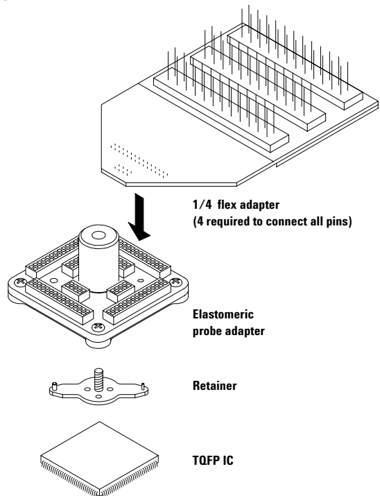
Figure 15. Elastomeric probing solution
