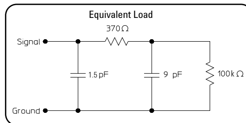
Figure 29. E5385A input equivalent load
