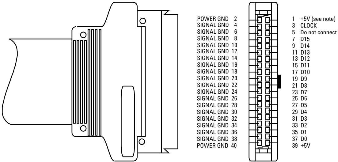
Figure 19. Pinout for probe cable
