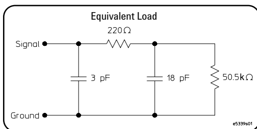
Figure 27. E5339A input equivalent load
