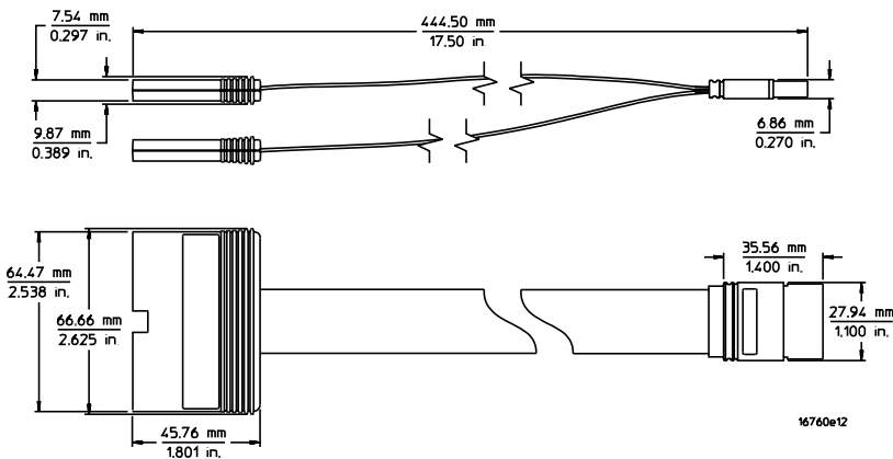
Figure 54. E5380A 38-Pin probe dimensions
