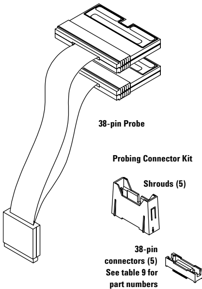
Figure 49. Agilent E5380A probe
