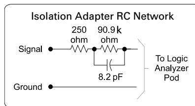
Figure 18. Isolation adapter (01650-63203) and equivalent load
