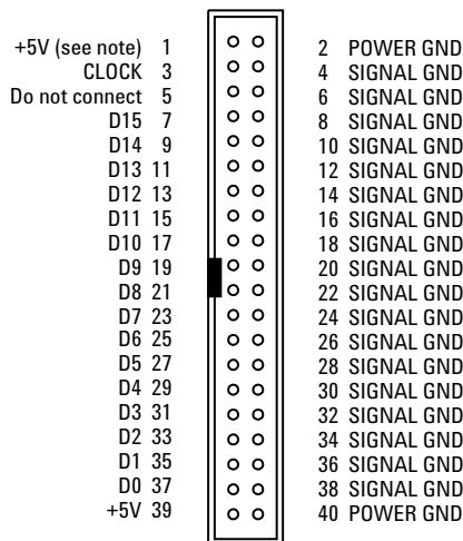
Figure 21. Forty-pin connector pinout
