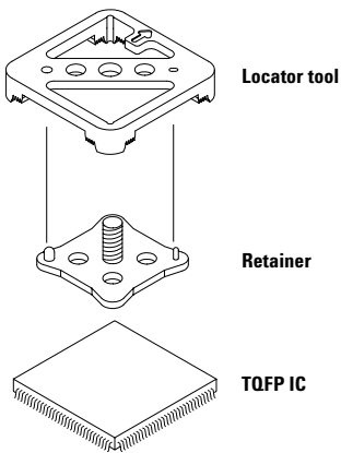
Figure 14. Locator tool aligning retainer on the device
