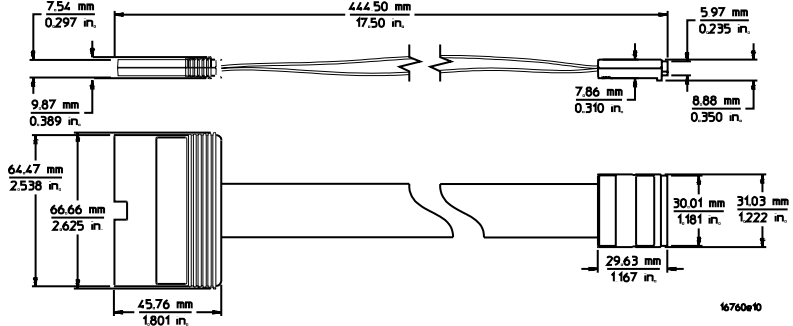
Figure 51. E5378A 100-pin single-ended probe dimensions
