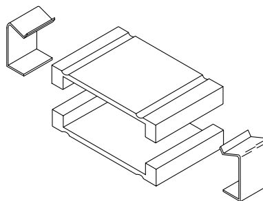
Figure 13. Ferrite core assembly, 16555-60001
