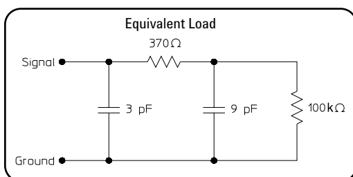
Figure 28. E5346A input equivalent load
