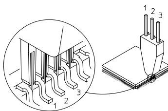
Figure 10. Three-signal Wedge electrical connection
