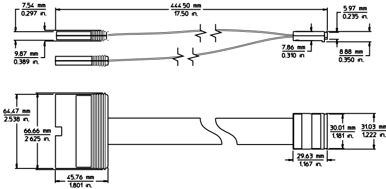
Figure 52. E5379A 100-pin differential probe dimensions
