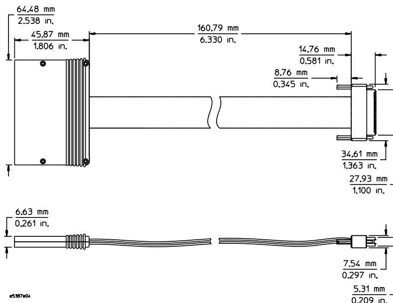
Figure 41. Soft touch probe (E5387A and E5390A) dimensions
