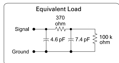
Figure 18. Isolation adapter (01650-63203) and equivalent load
