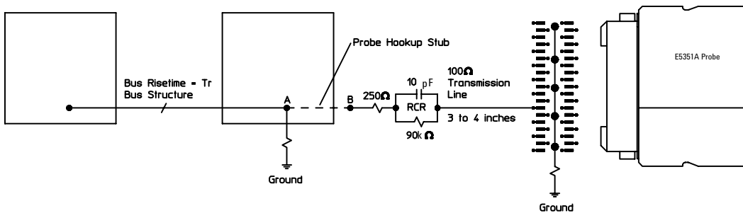
Figure 33. Agilent Technologies E5351A design rules
