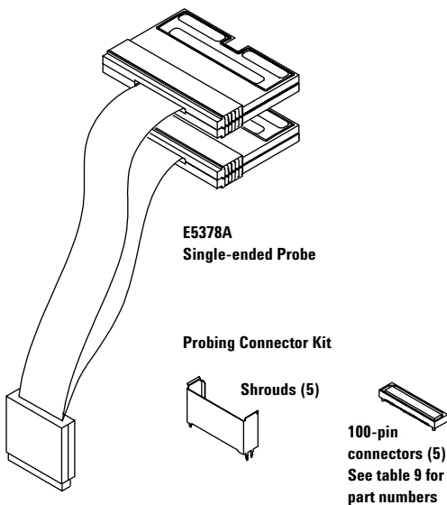
Figure 44. Agilent E5378A probe
